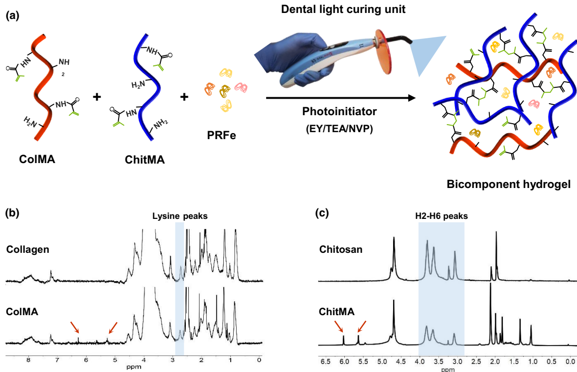
FIGURE 2 Synthesis and ^1\text{H} NMR analysis of extract of platelet-rich fibrin (PRFe)-loaded ChitMA/ColMA hydrogels. (a) Schematic representation of synthesis and photocrosslinking of the PRFe-loaded bicomponent hydrogels. (b) ^1\text{H} NMR spectra of non-modified collagen and ColMA. (c) ^1\text{H} NMR spectra of non-modified chitosan and ChitMA. Red arrows show the characteristic peaks of methacrylate moieties. ^1\text{H} NMR, proton nuclear magnetic resonance; ChitMA, methacrylated chitosan; ColMA, methacrylated collagen.
